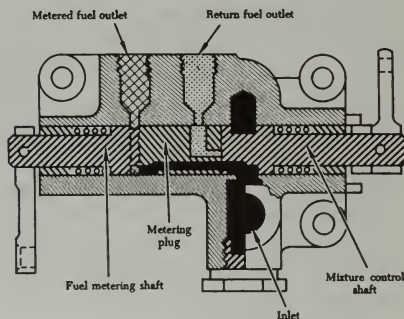
FIGURE 3-37. Fuel control assembly.
